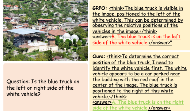
Figure 3. Case study of the visual reasoning process from models trained with GRPO and our method.
