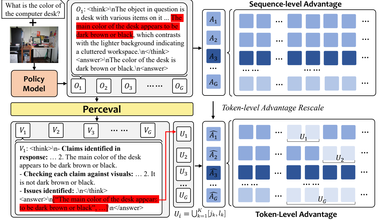
Figure 1. An overview of our Process-Supervised GRPO framework. For each generated response, we use the Perceval to create a token-level penalty mask. This mask is used to calculate a fine-grained token-level advantage, which is then incorporated into the GRPO objective to penalize hallucinatory tokens and improve the model’s perceptual grounding.
