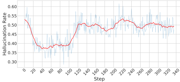
Figure 2. The proportion of responses identified by PERCEVAL as containing hallucinations during training.
